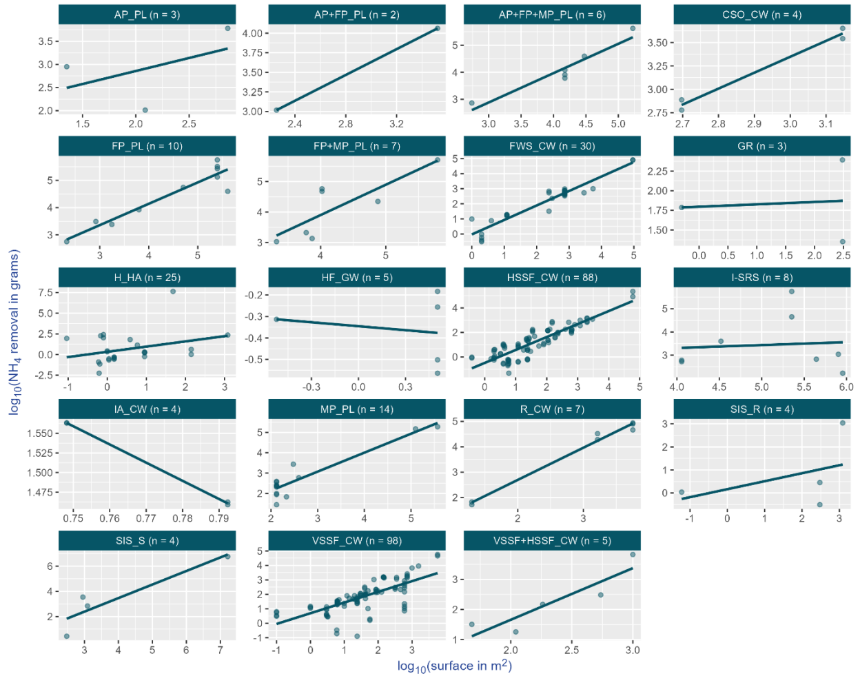
Figure 11. NH 4 removal as a function of surface using power models.
