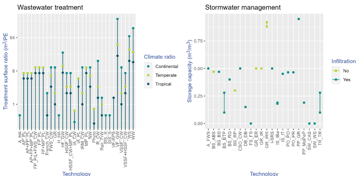
Figure 5. Expert-based data used to estimate the required surface for wastewater treatment (left) and stormwater management (right) technologies. Note that the scale in left panel is in log 2 . The acronyms description can be found in Appendix 1.
